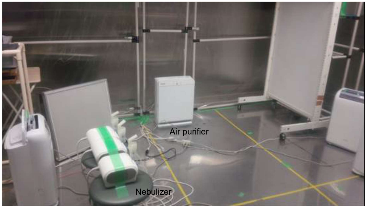
Fig. 2 Condition of installation of home air purifier MA-E85K
