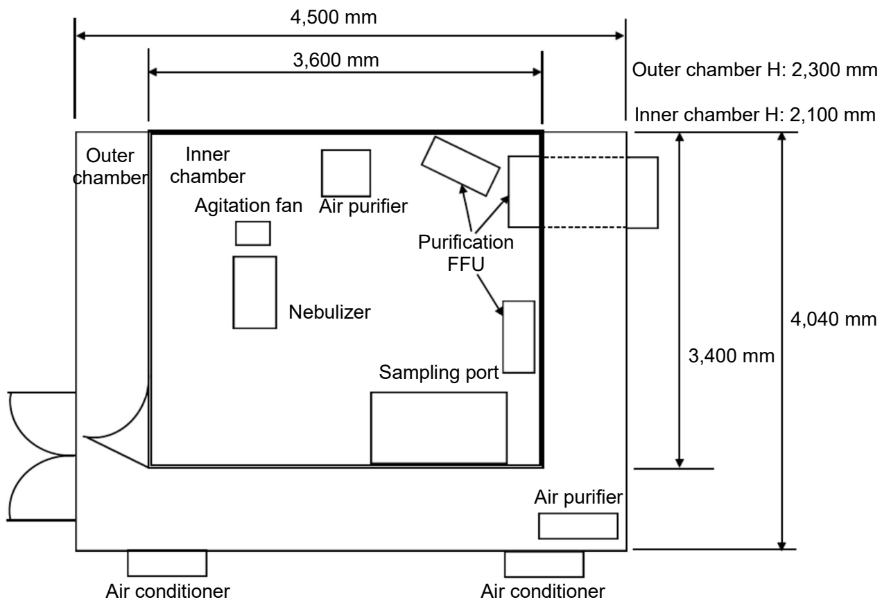
Fig. 1 Test chamber and condition of installation of various devices
